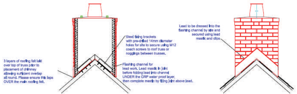
Section view along ridge
