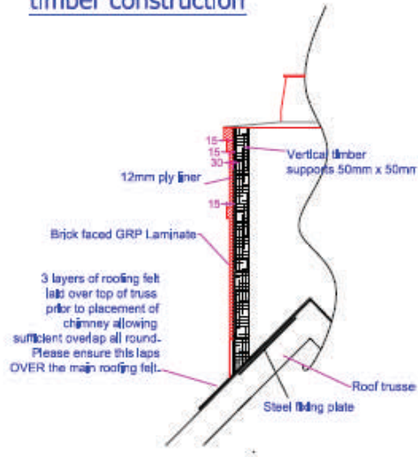
Section view along ridge
